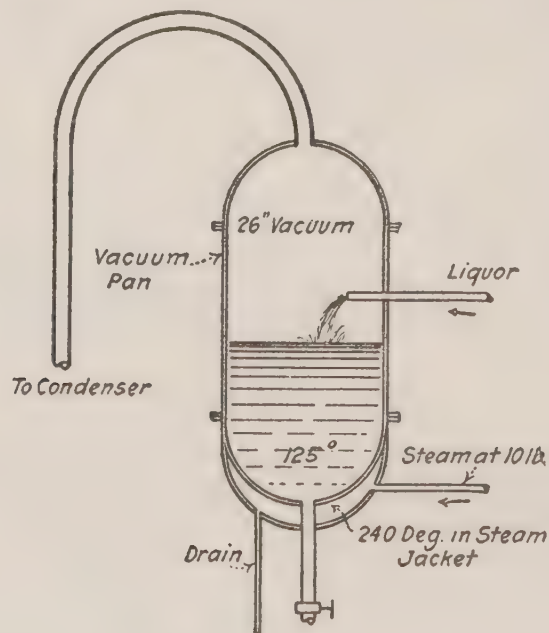
FIG. 8 VACUUM PAN
